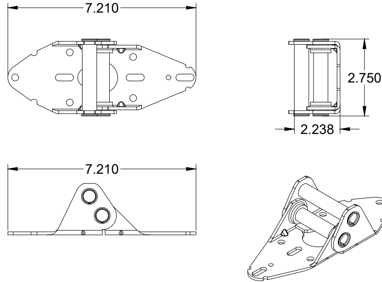
#4 ROLLER HINGE
