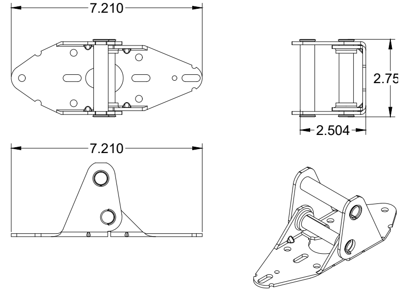
#5 ROLLER HINGE
